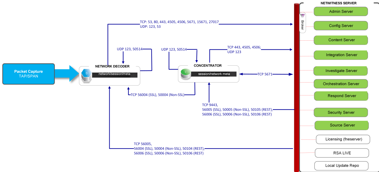
NetWitness Network 11.7 Architecture with Ports
