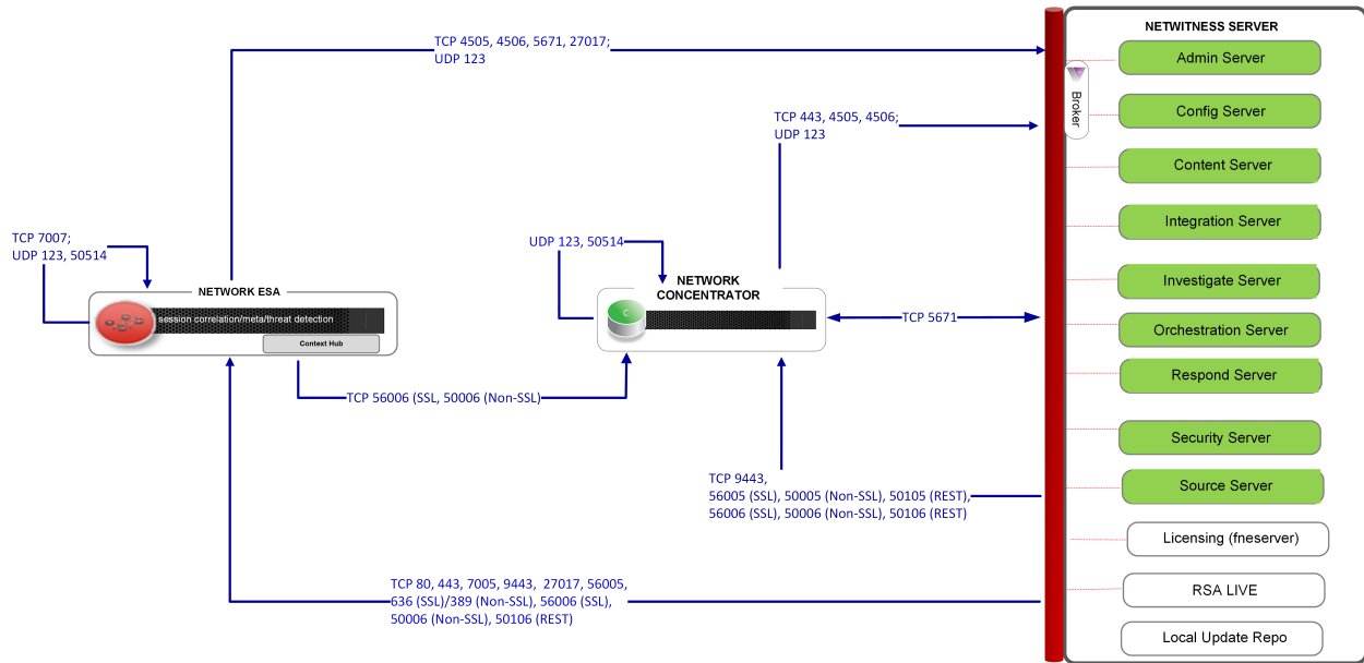
Event Source Analysis (ESA) Network 11.7 Architecture with Ports
