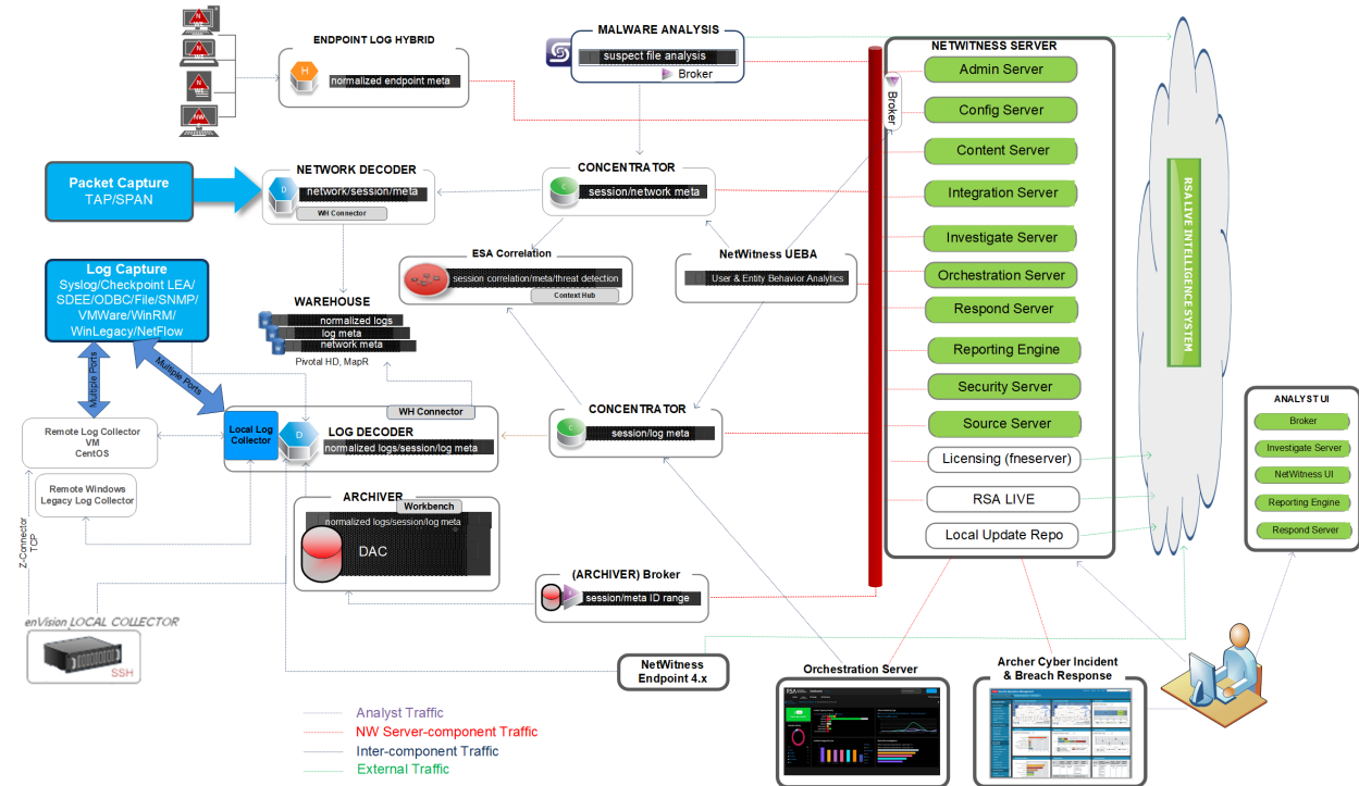
Global NetWitness Platform 11.4 Architecture
