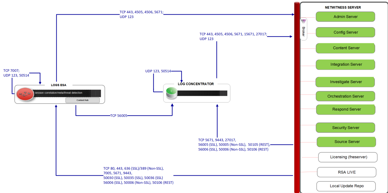
Event Source Analysis (ESA) Logs 11.4 Architecture with Ports
