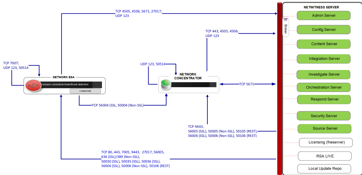
Event Source Analysis (ESA) Network 11.4 Architecture with Ports
