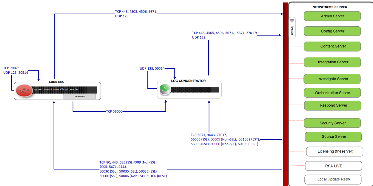
Event Source Analysis (ESA) Logs 11.5 Architecture with Ports
